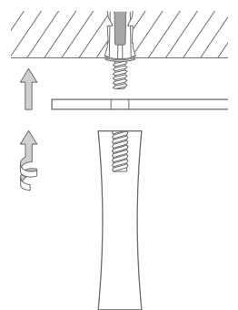
Montage HL3F / HL5F:
