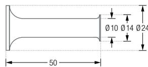
HG24-50:
