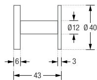
HA1-R40S40:
