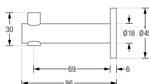
H18-80K45:
