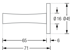
HF16-65K45:
