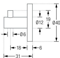
H12-25E-K40:
