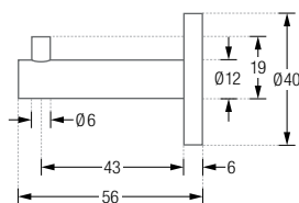
H12-50E-K40:
