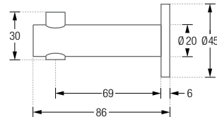
H20-80K45:
