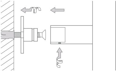
Montage GSTR-W-B:
