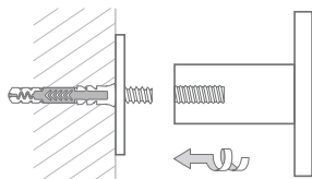
Montage HA3-R40S55-B:
