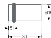
HG15-30-B:
