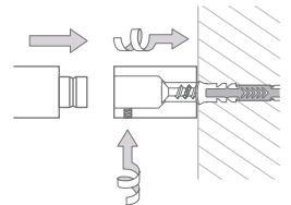
Montage HLS3H-B / HLS5H-B:
