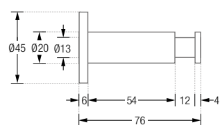
HN20-70K45:
