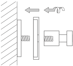
Montage HN16-30K45:
