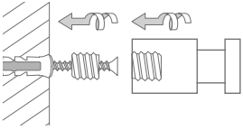
Montage HN16-30K45:
