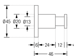
HN20-40K45:
