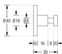
HN16-30K45:
