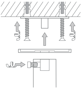
Montage HS26:
