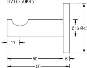
HV16-50K45:
