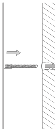
Montage BFSS-Set2:
