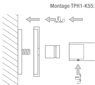
Montage TPH1-K55:
